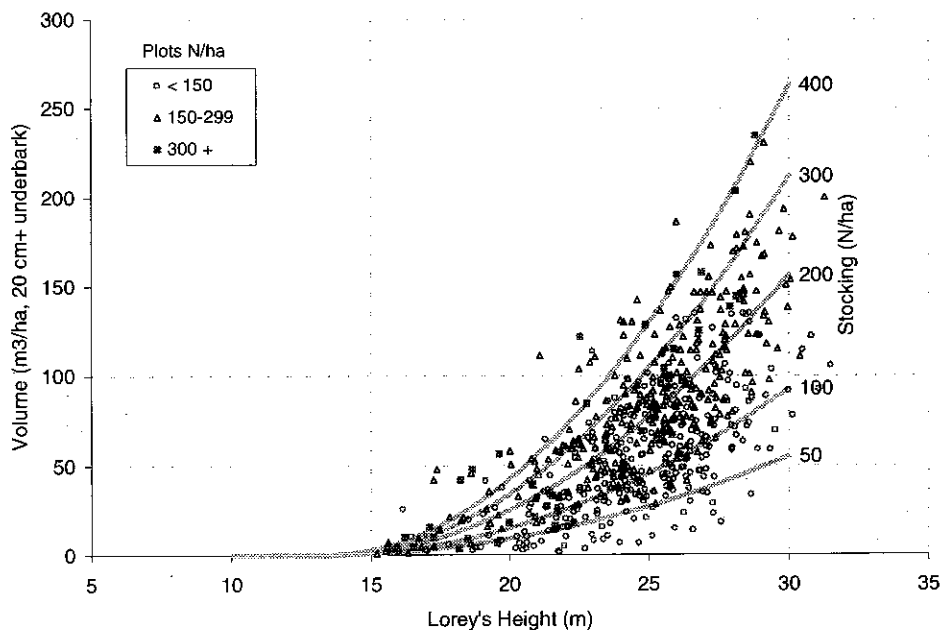
FIGURE 5 Model of volume underbark to 20 cm top diameter as a function of stocking and height
