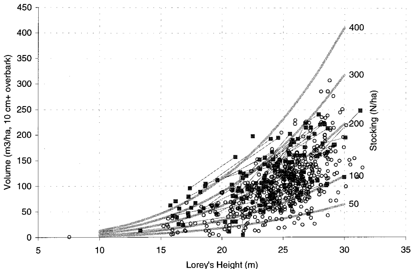
FIGURE 3 Model relating stand volume, Lorey's height and stocking [TSPs shown as circles, PSPs as connected squares, model as thick lines]
