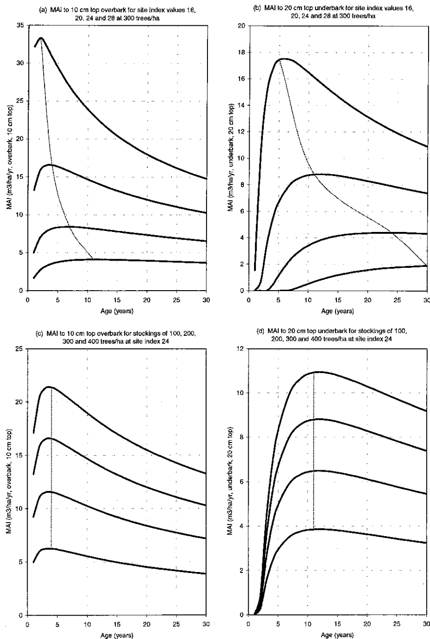
FIGURE 6 MAI curves for different site indexes and stockings, for volume to 10 cm top overbark (left) and 20 cm top underbark (right)
