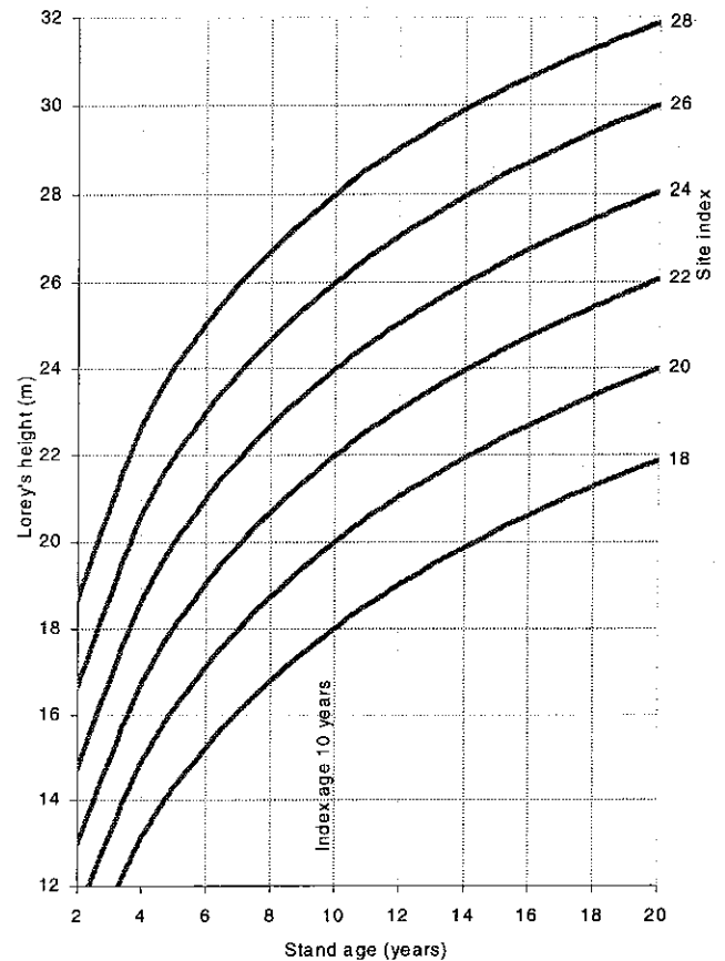
FIGURE 2 Site index curves for Cordia alliodora in Ecuador based on equation 4
