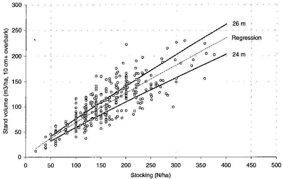
FIGURE 4 Stand volume against stocking for plots with Lorey's height between 23 and 27 m [The thick lines are calculated from equation {7} for heights of 24 and 26 m. The thin line is a regression fitted to the data shown.]
